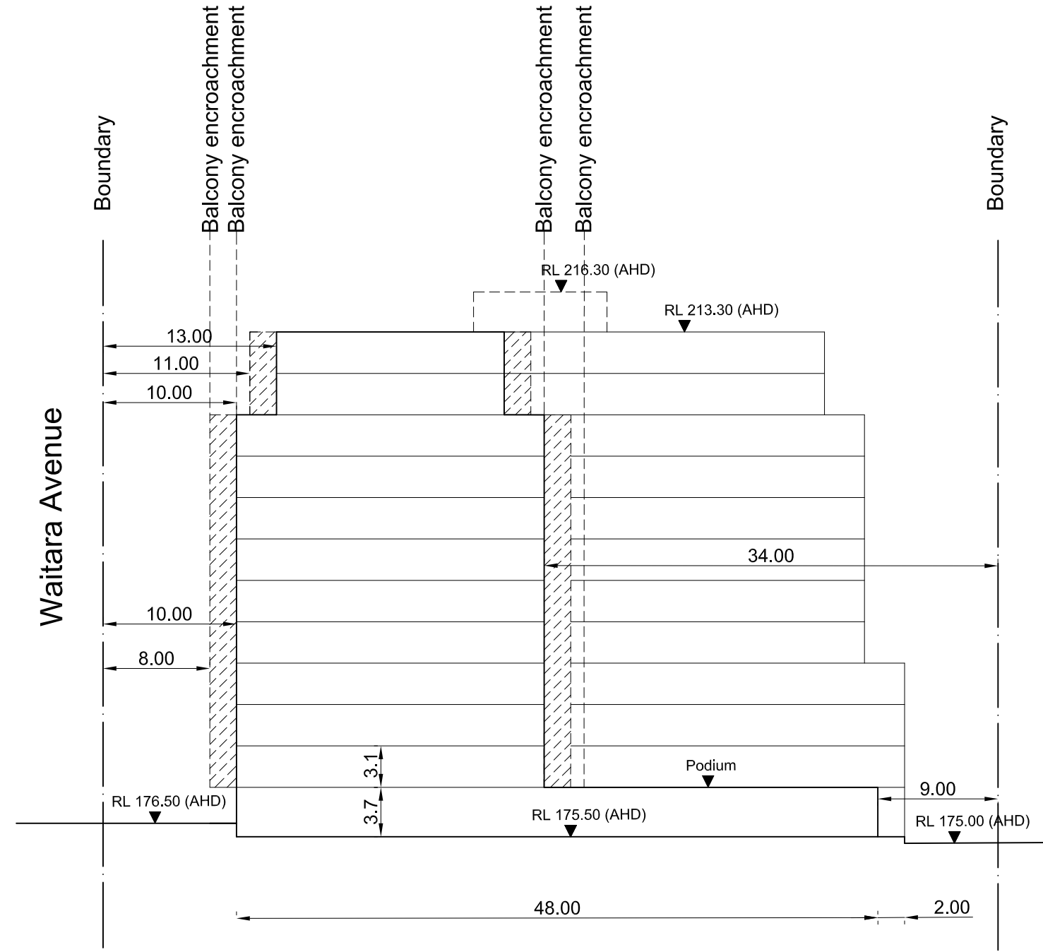
Section BB
