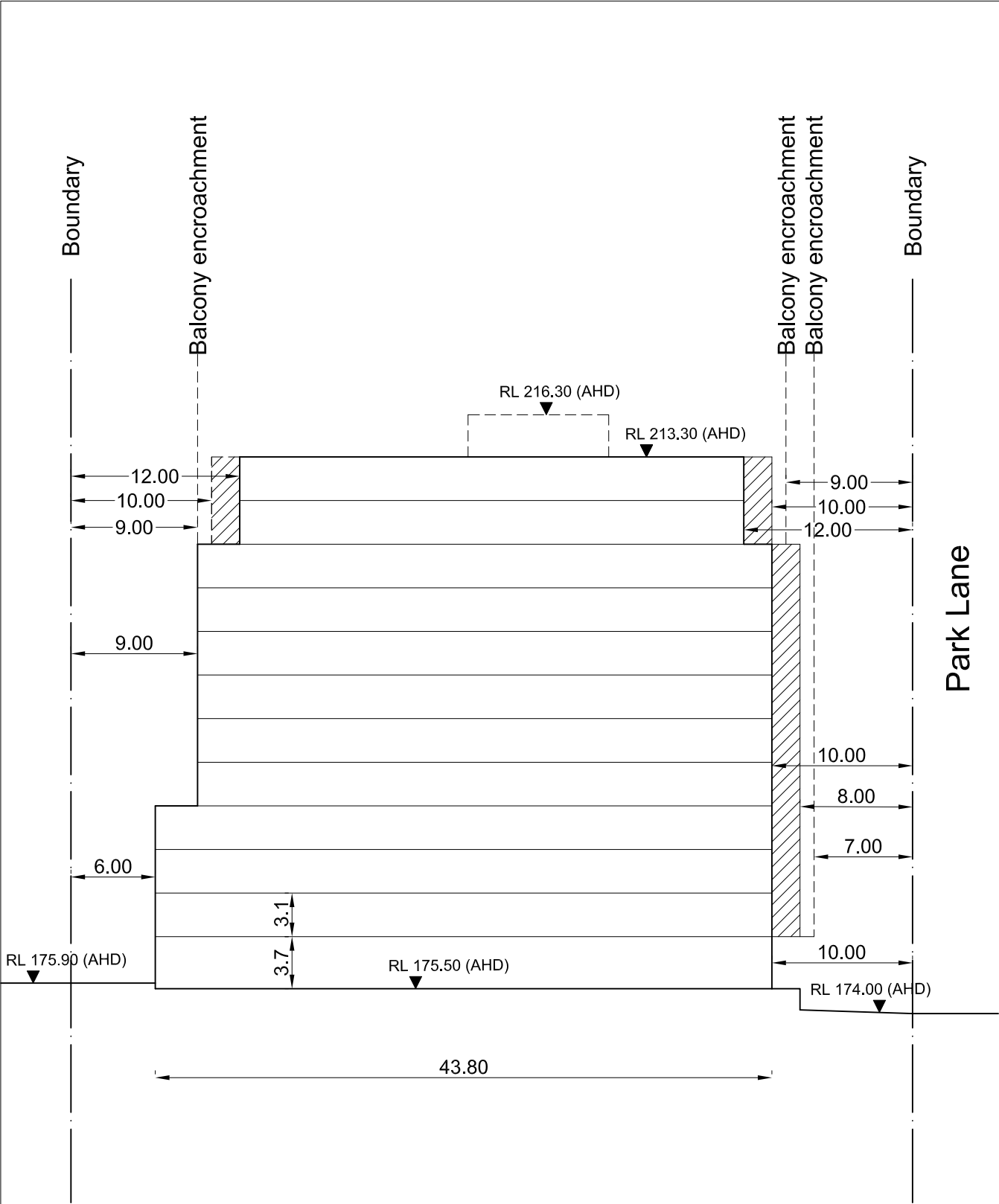
Section CC
